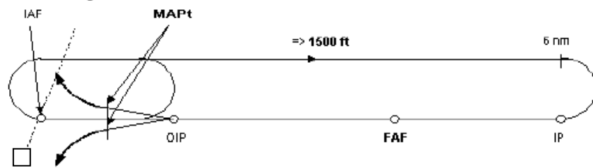
Figure 4 - Holding Pattern &amp; Race Track Procedure
